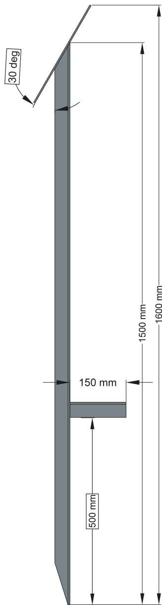
T-stål like bent 40x40x4 mm
