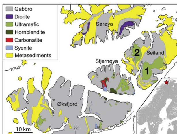
Figure 1: Map of the Seiland Igneous Province modified from Larsen et al., (2018). Inset shows location of SIP in northern Norway. Primary targets for field work in summer 2023 within Seiland National Park are labeled: 1 – Melkvann Ultramafic Complex 2 – Nordre Brummansfjord Ultramafic Complex
